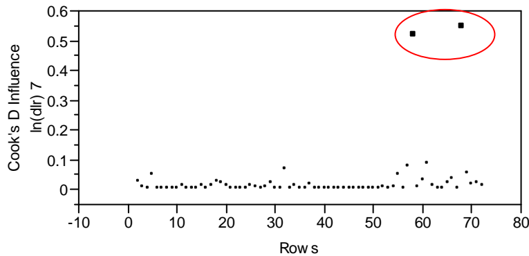
Figure 16: Overlay Plot of Cook's Distance Values for Model 3
