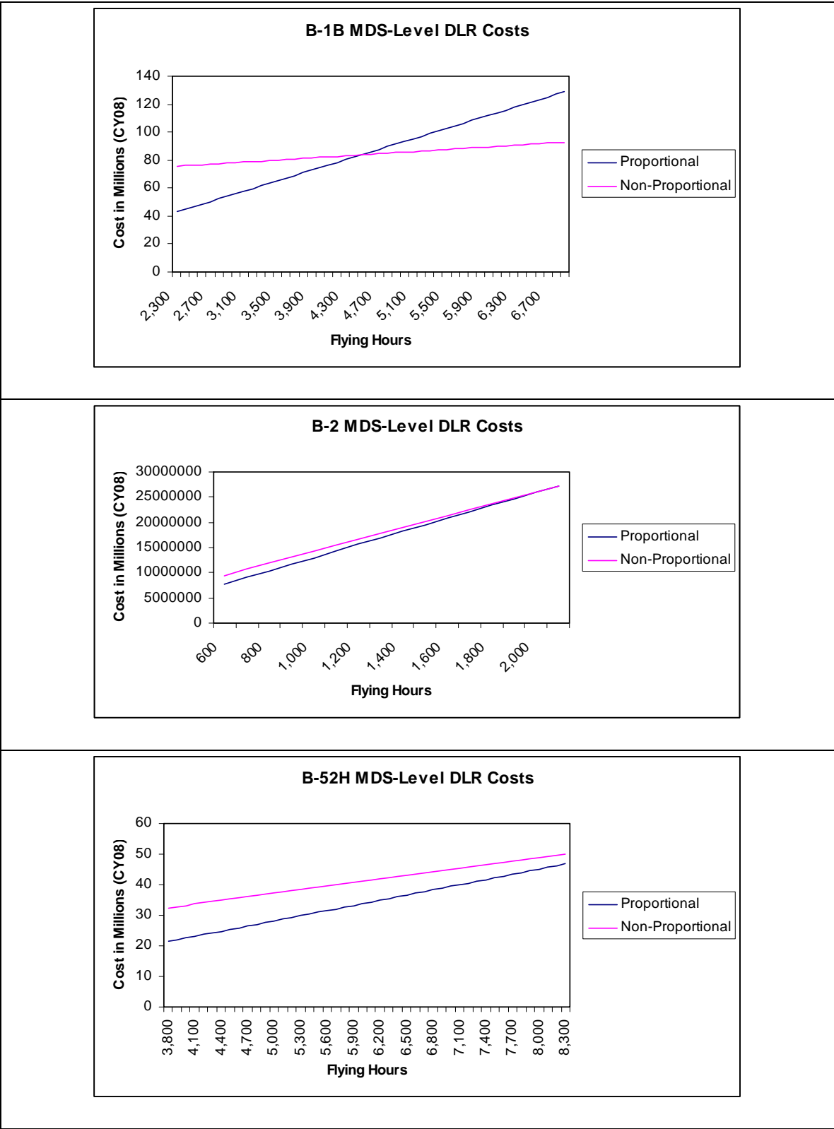
Figure 6: Proportional Forecasts versus Non-Proportional Forecasts for DLR Costs
