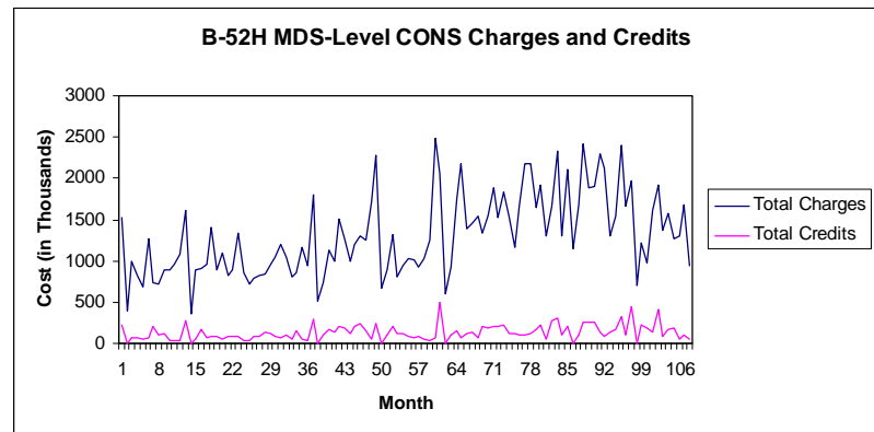
Figure 23: CONS Charges and Credits Over Time
