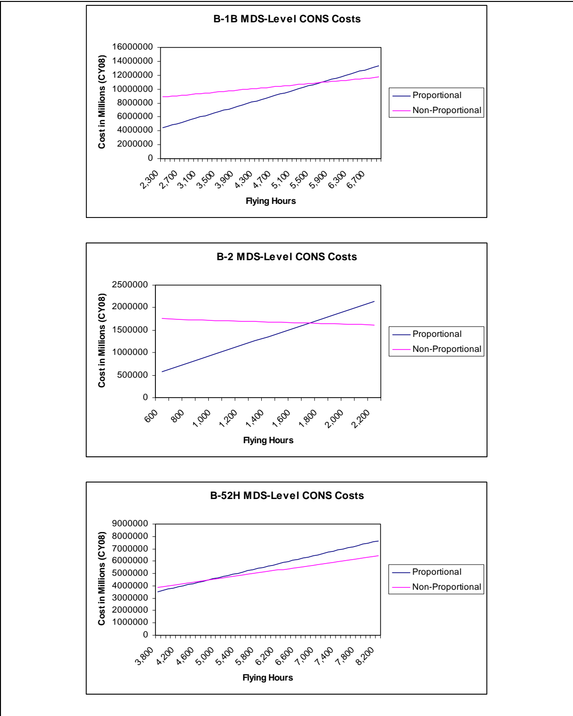
Figure 7: Proportional Forecasts versus Non-Proportional Forecasts for CONS Costs
